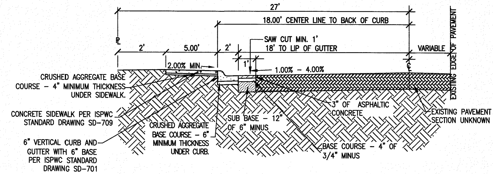
2 Proposed Pavement Match And New Curb, Gutter And Sidewalk In South Sailer Place
