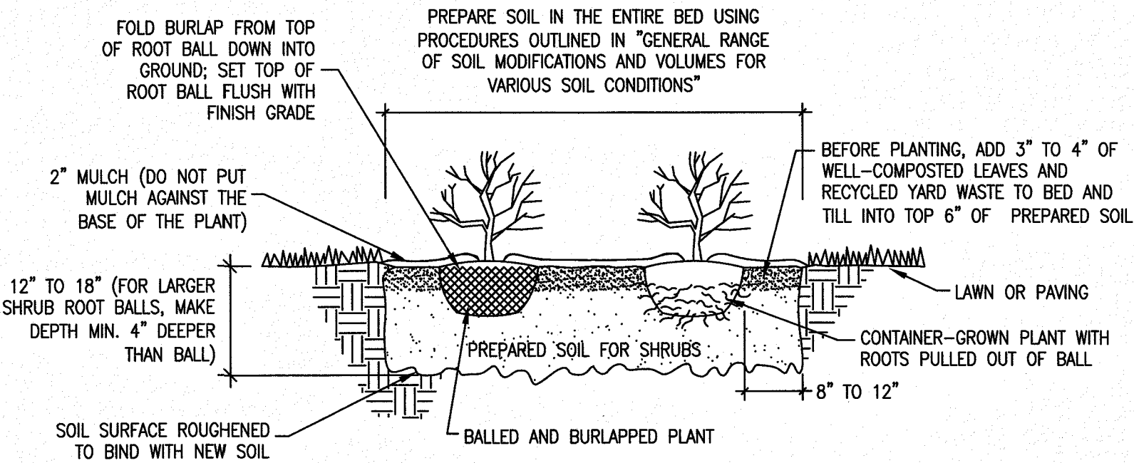
Typical Shrub Planting Detail
