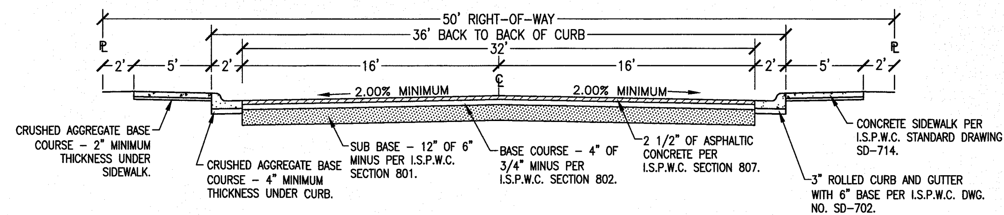
1 Proposed Sailer Shores Lane Cross-section
