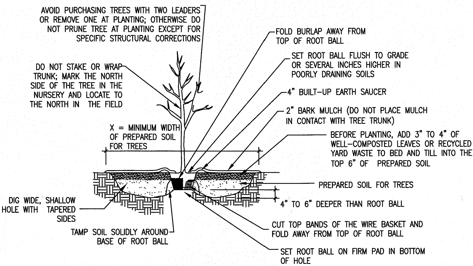
Typical Tree Planting Detail
